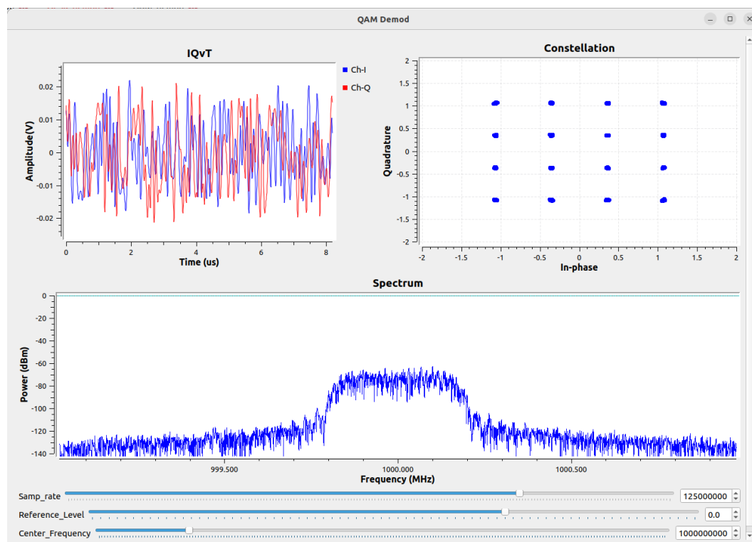
Figure 7-1 QAM demodulation example
