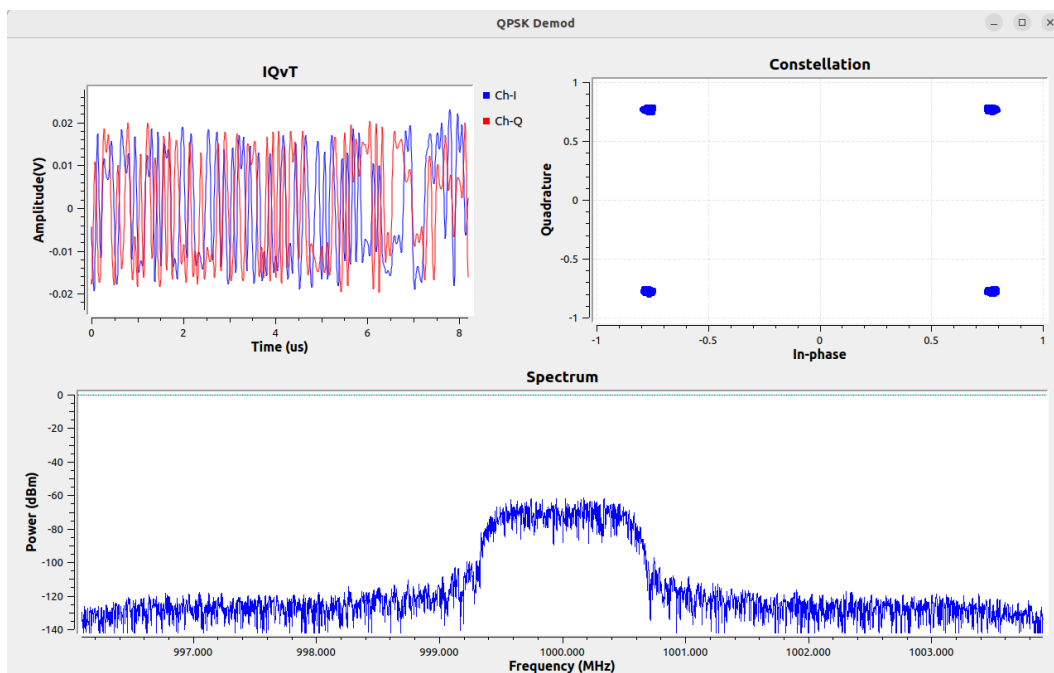
Figure 17 QPSK demodulation example
