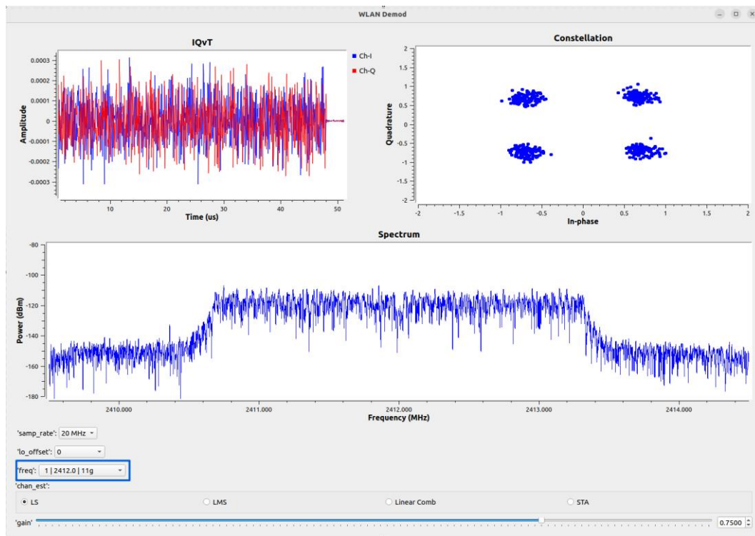
Figure 18 WLAN demodulation example
