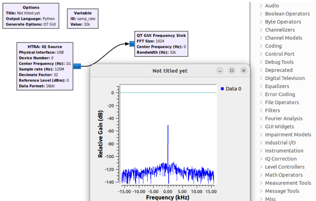
Figure 12 Viewing the Input Signal Spectrum
