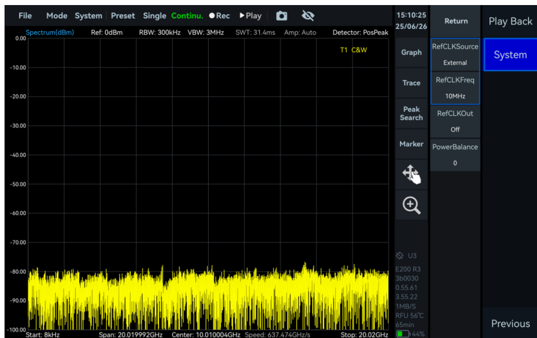
Figure 54 Use an external 10 MHz reference clock
