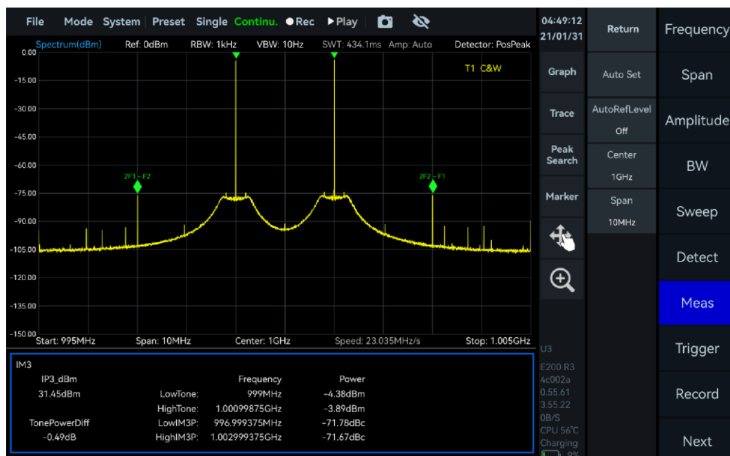
Figure 27 Measurement of IP3/IM3
