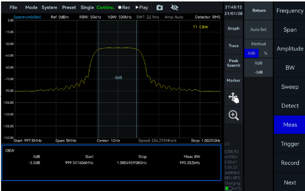
Figure 25 Measurement of OBW
