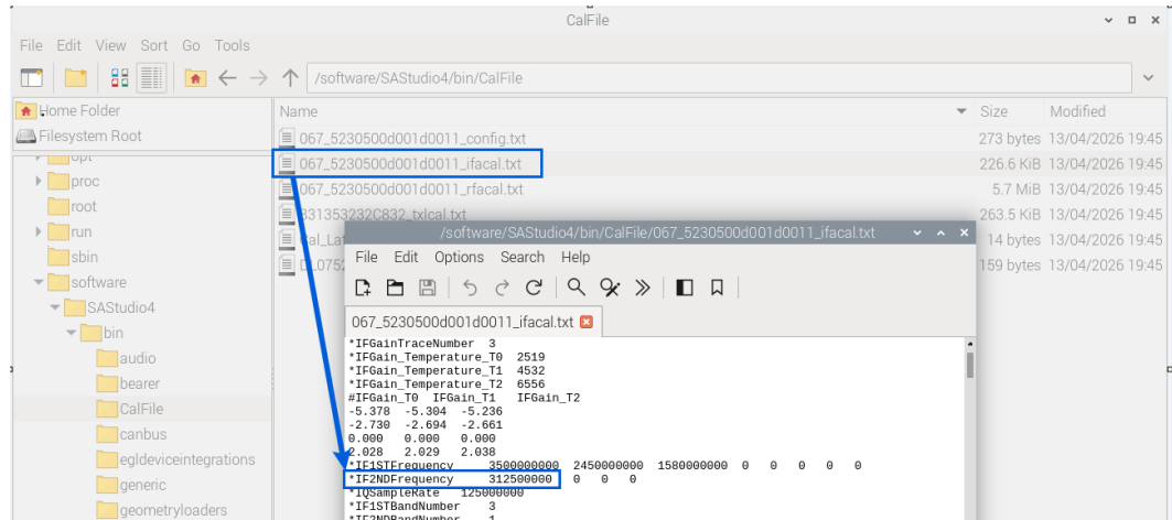
Figure 53 Check the IF Output Center Frequency on PXN Series Instruments
