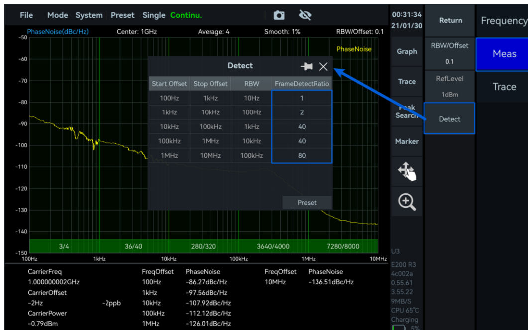
Figure 46 Pulse Signal Detection Settings
