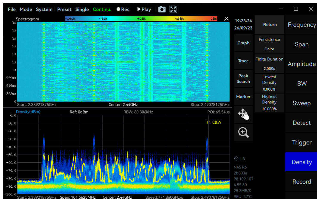
Figure 43 Probability Density Display of a Wi-Fi Signal
