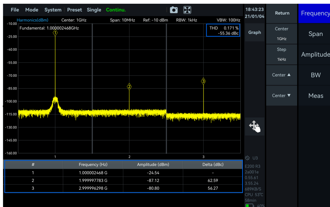
Figure 45 Measurement of Third Harmonic
