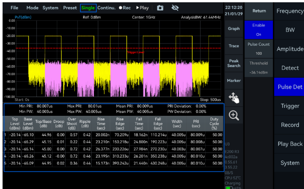
Figure 40 Result of Pulse Detection
