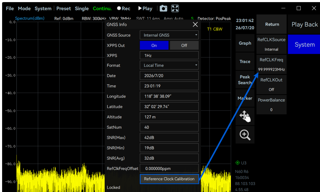
figure 10 Reference Clock Calibration
