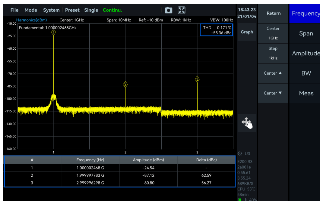
Figure 44 Measurement of Third Harmonic
