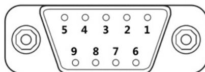
Figure 11 EIO Expansion Board Interface Diagram
