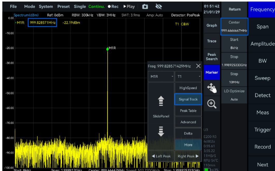
Figure 17 Frequency Tracking
