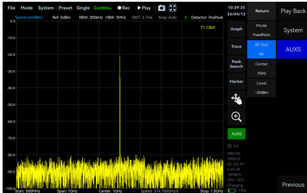
Figure 47 AUXS Single-Tone Signal Output
