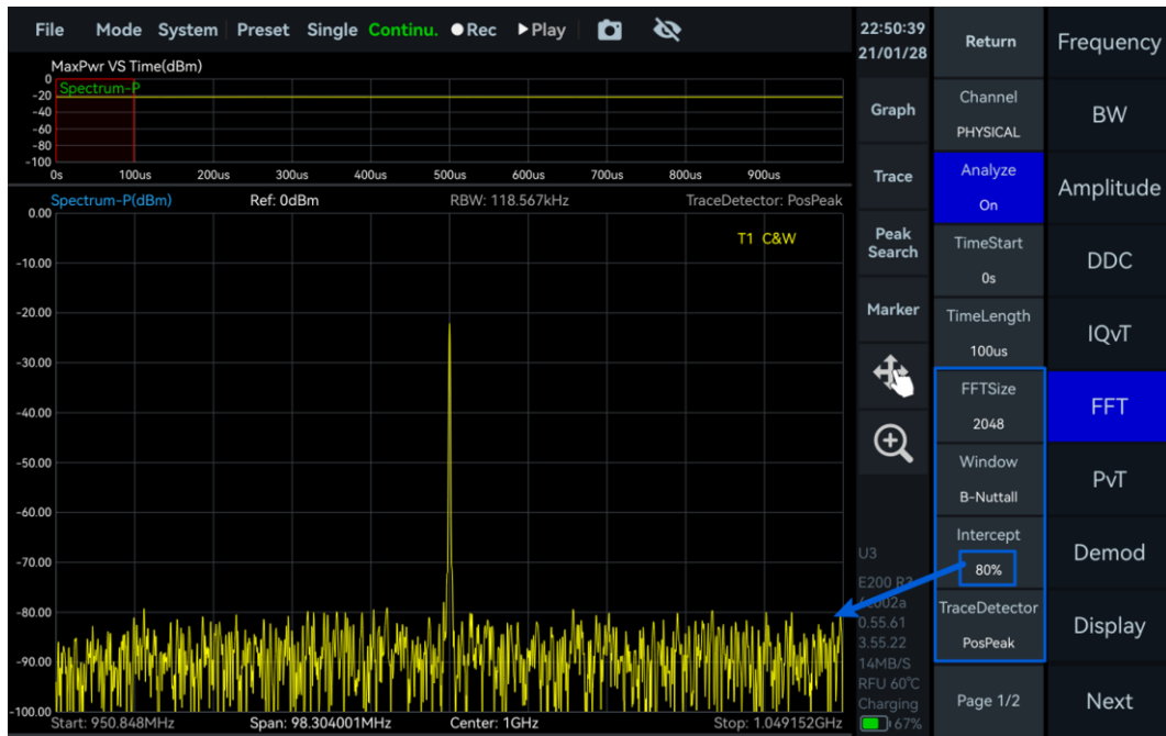
Figure 31 Spectrum analysis of IQ data
