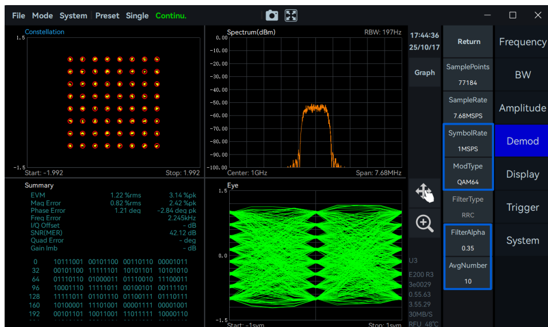
Figure 43 64QAM Demodulation
