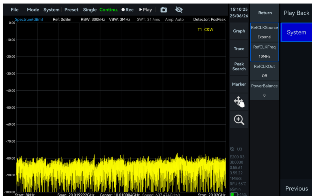
Figure 53 Use an external 10 MHz reference clock
