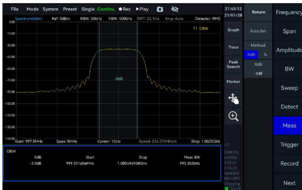
Figure 24 Measurement of OBW
