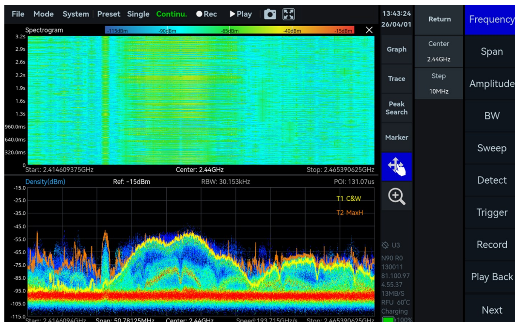
Figure 42 Probability Density Plot of WIFI Signal
