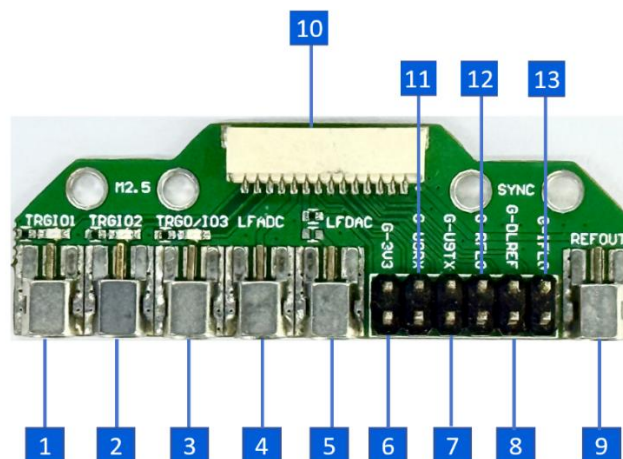
Figure 13-2 R1000 Series Trigger Board Interface Diagram
