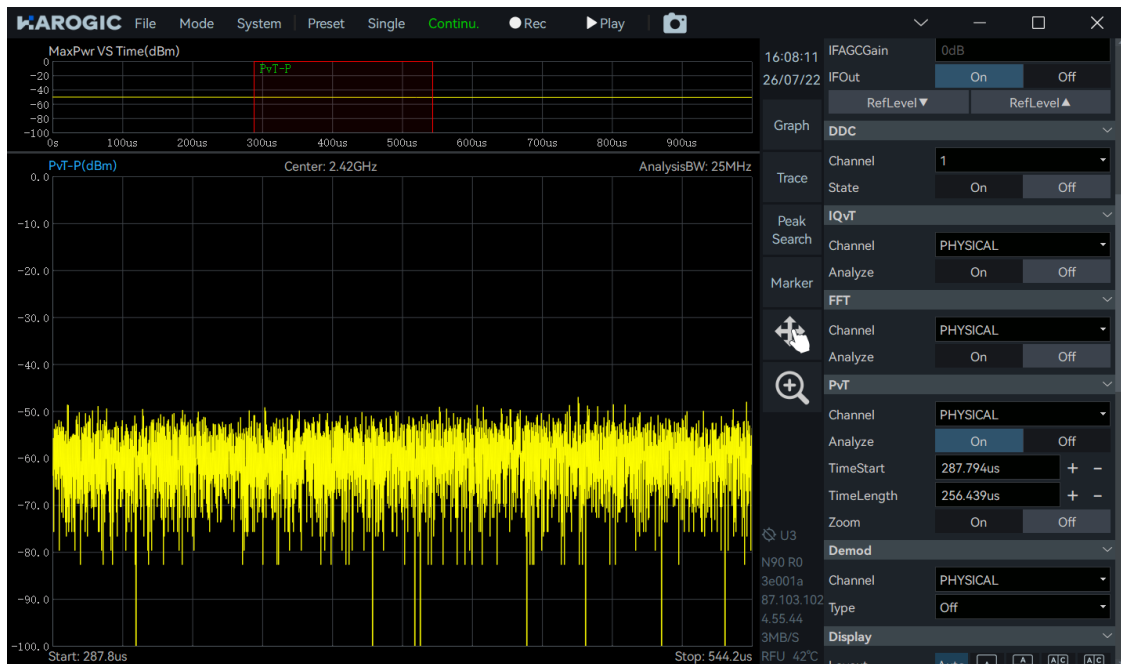
Figure 8-4 PvT Waveform in Receiver IQ Streaming Mode
