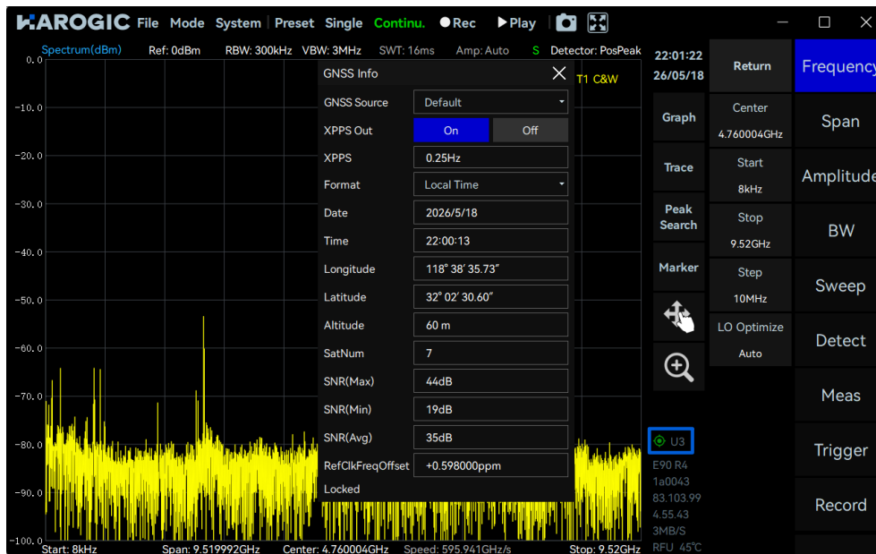
Figure 12- 3 Lock the GNSS External Antenna
