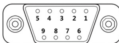
Figure 13-3 EIO Expansion Board Interface
