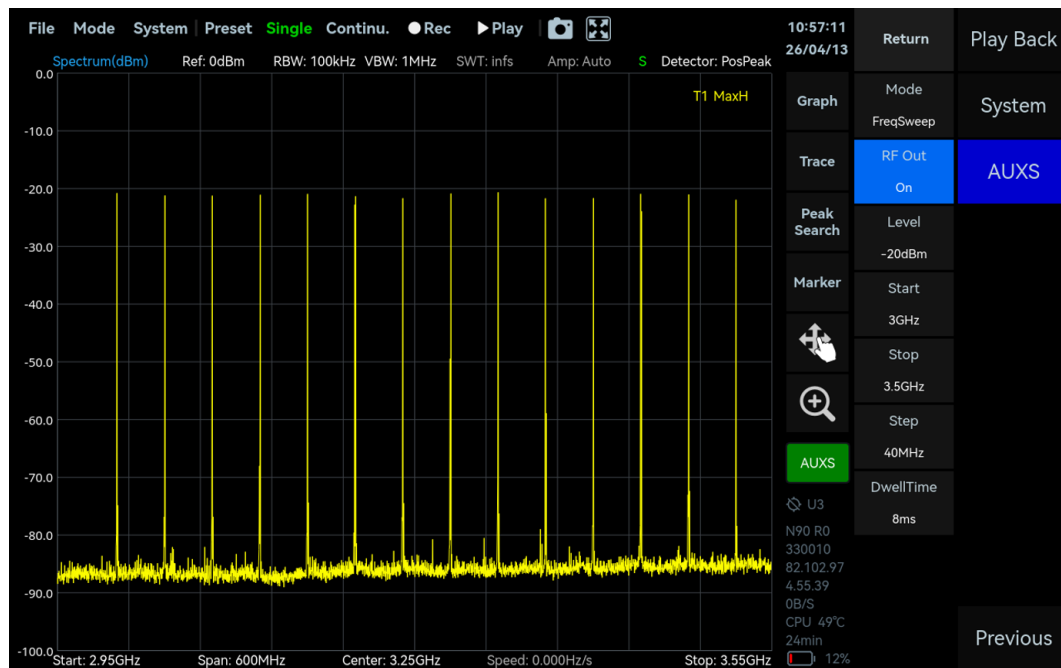
Figure 50 AUXS Frequency Sweep Signal Output
