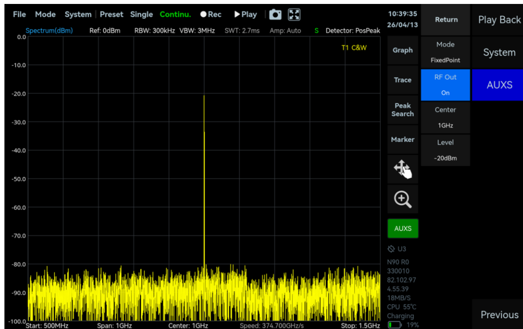
Figure 49 AUXS Single-Tone Signal Output
