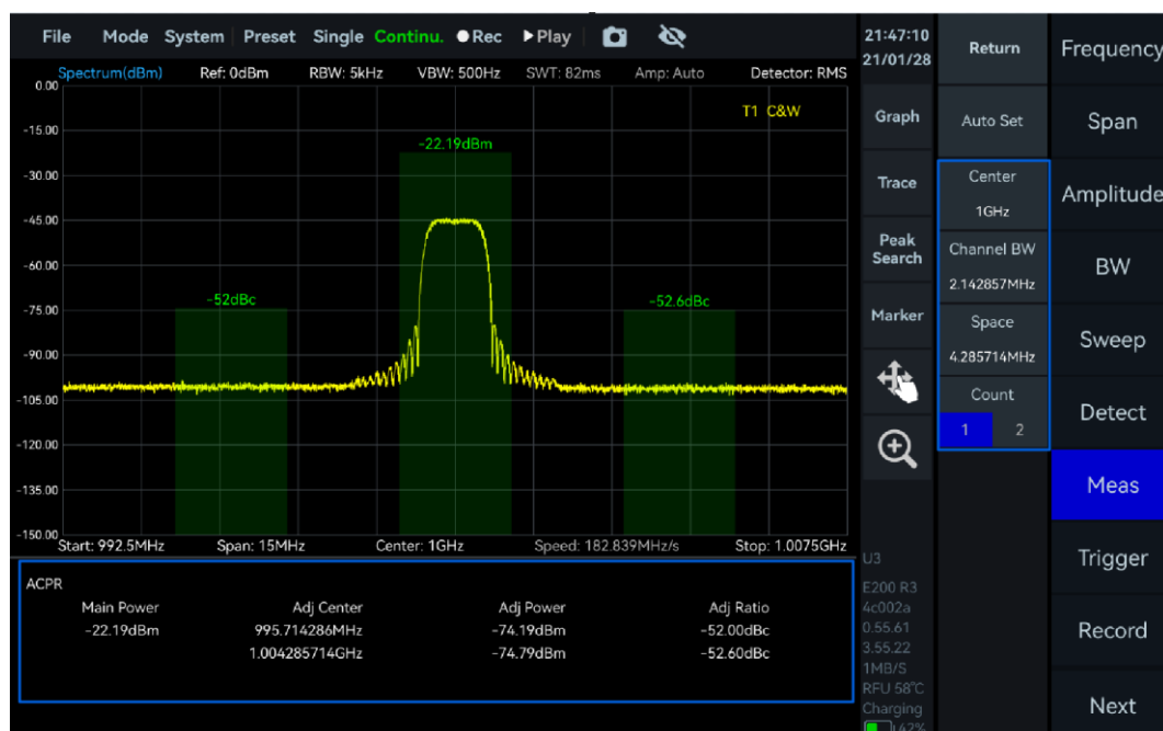
Figure 25 Measurement of ACPR
