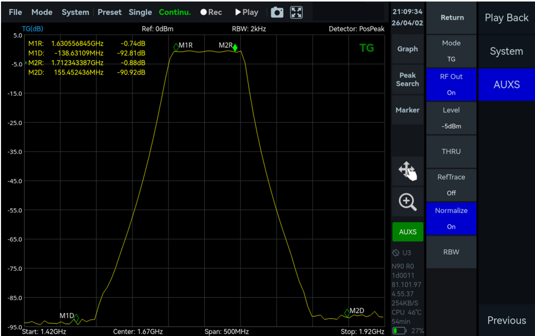
Figure 51 Frequency response curve of a band-pass filter
