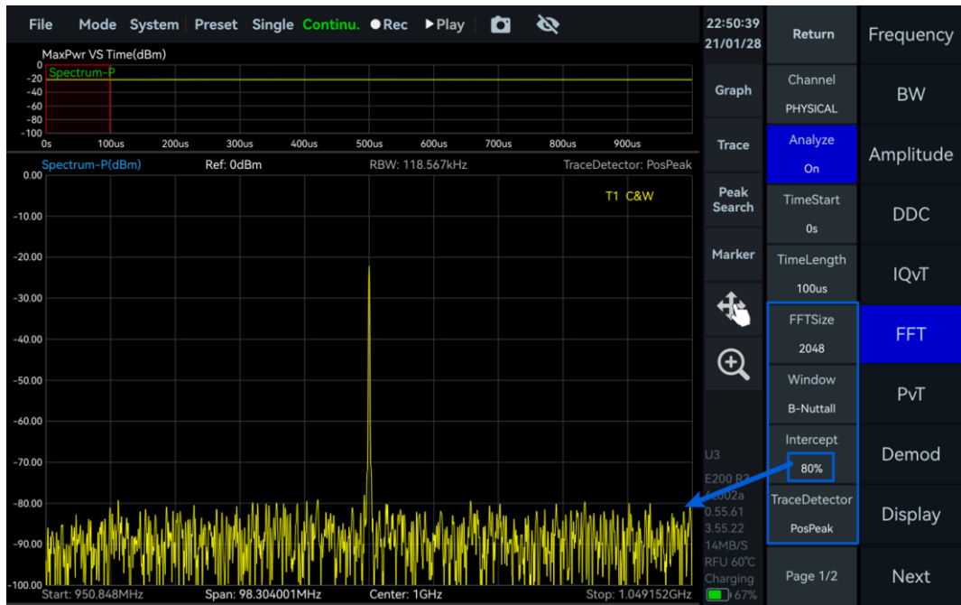
Figure 31 Spectrum analysis of IQ data
