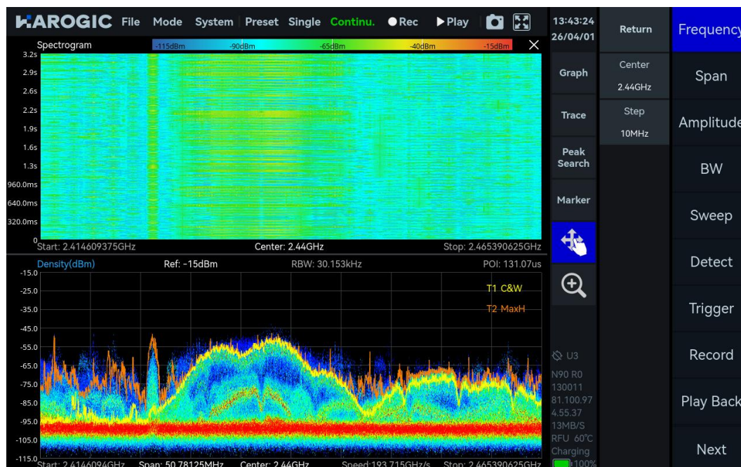
Figure 40 Probability Density Plot of WIFI Signal
