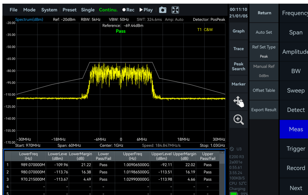
Figure 25 Measurement of SEM
