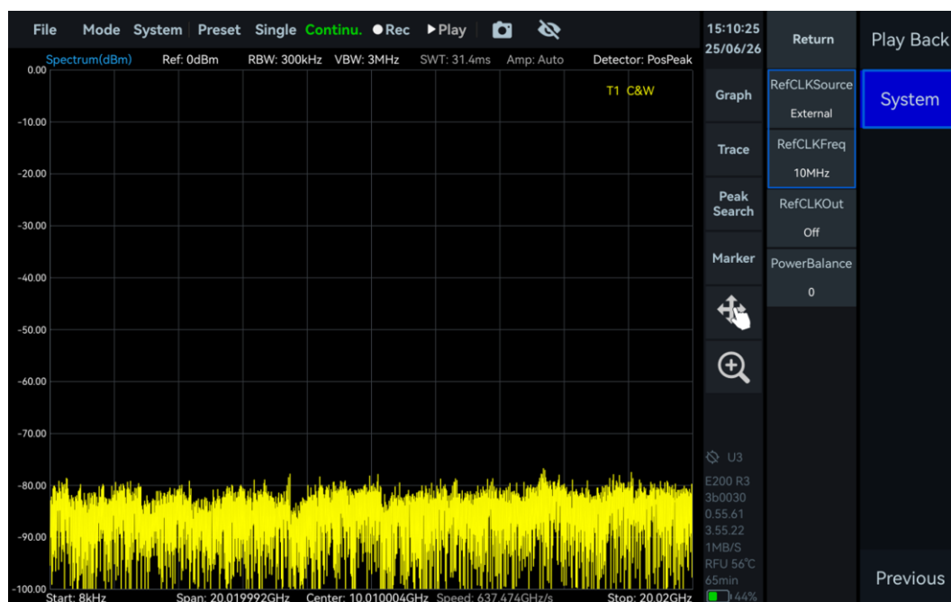
Figure 51 Use an external 10 MHz reference clock
