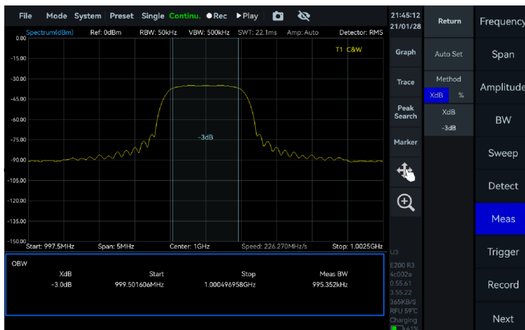
Figure 22 Measurement of OBW
