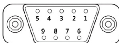
Figure 9 EIO Expansion Board Interface Diagram
