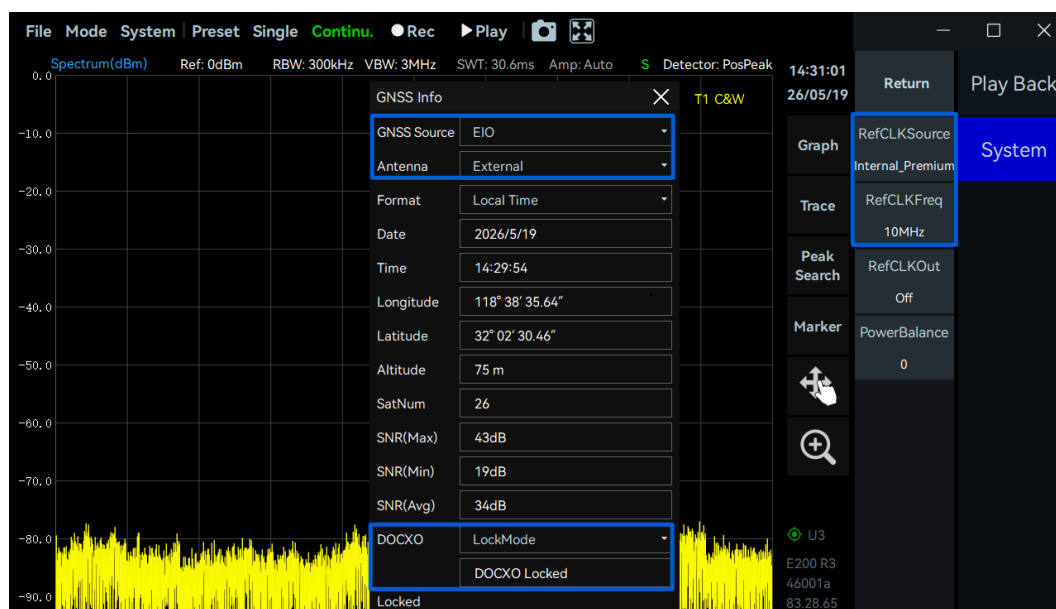
Figure 7 10MHz reference clock using high quality GNSS modules
