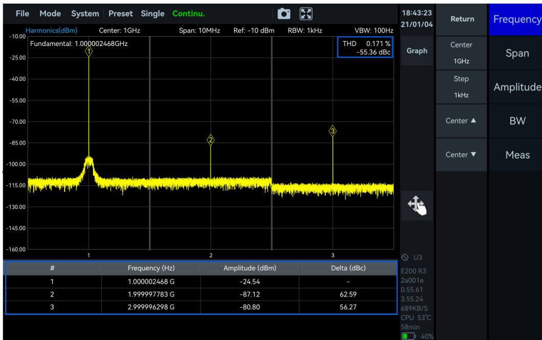
Figure 42 Measurement of Third Harmonic
