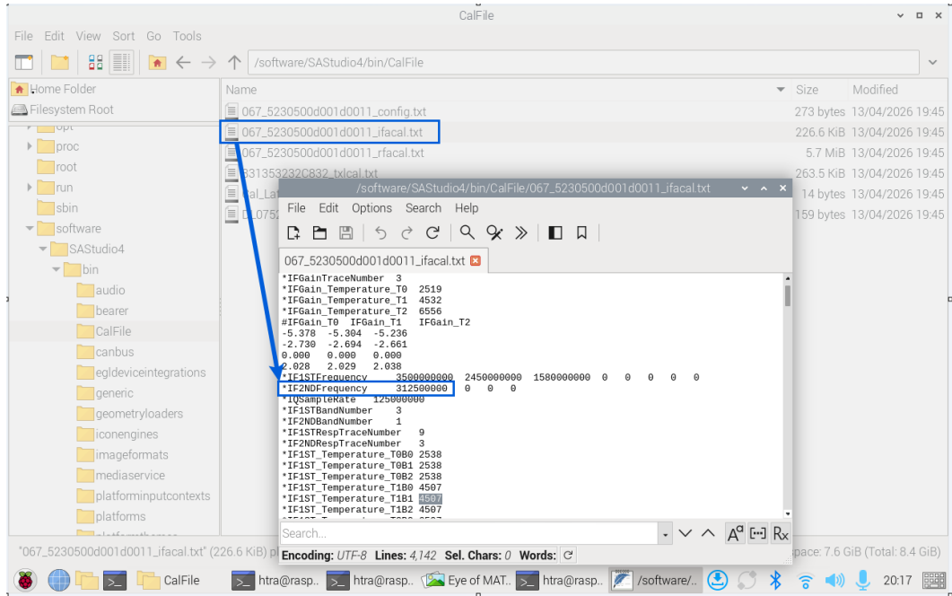
Figure 49 Check the IF Output Center Frequency on PXN Series Instruments
