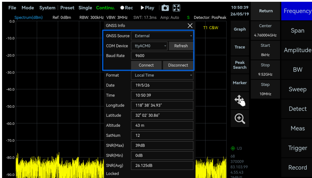
Figure 8 Connecting an external GNSS module
