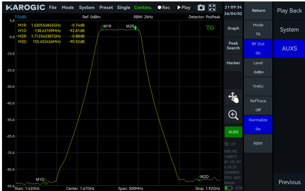
Figure 48 Frequency response curve of a band-pass filter
