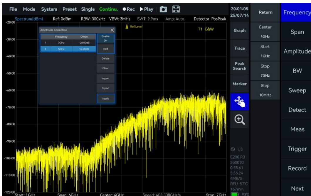
Figure 18 Amplitude correction application
