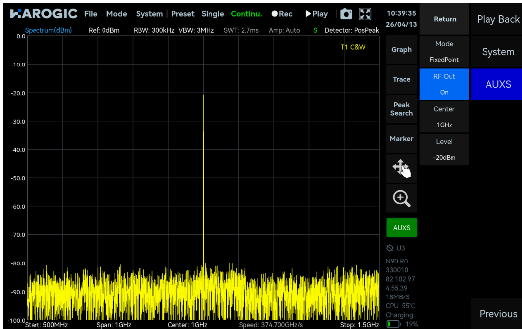
Figure 46 AUXS Single-Tone Signal Output
