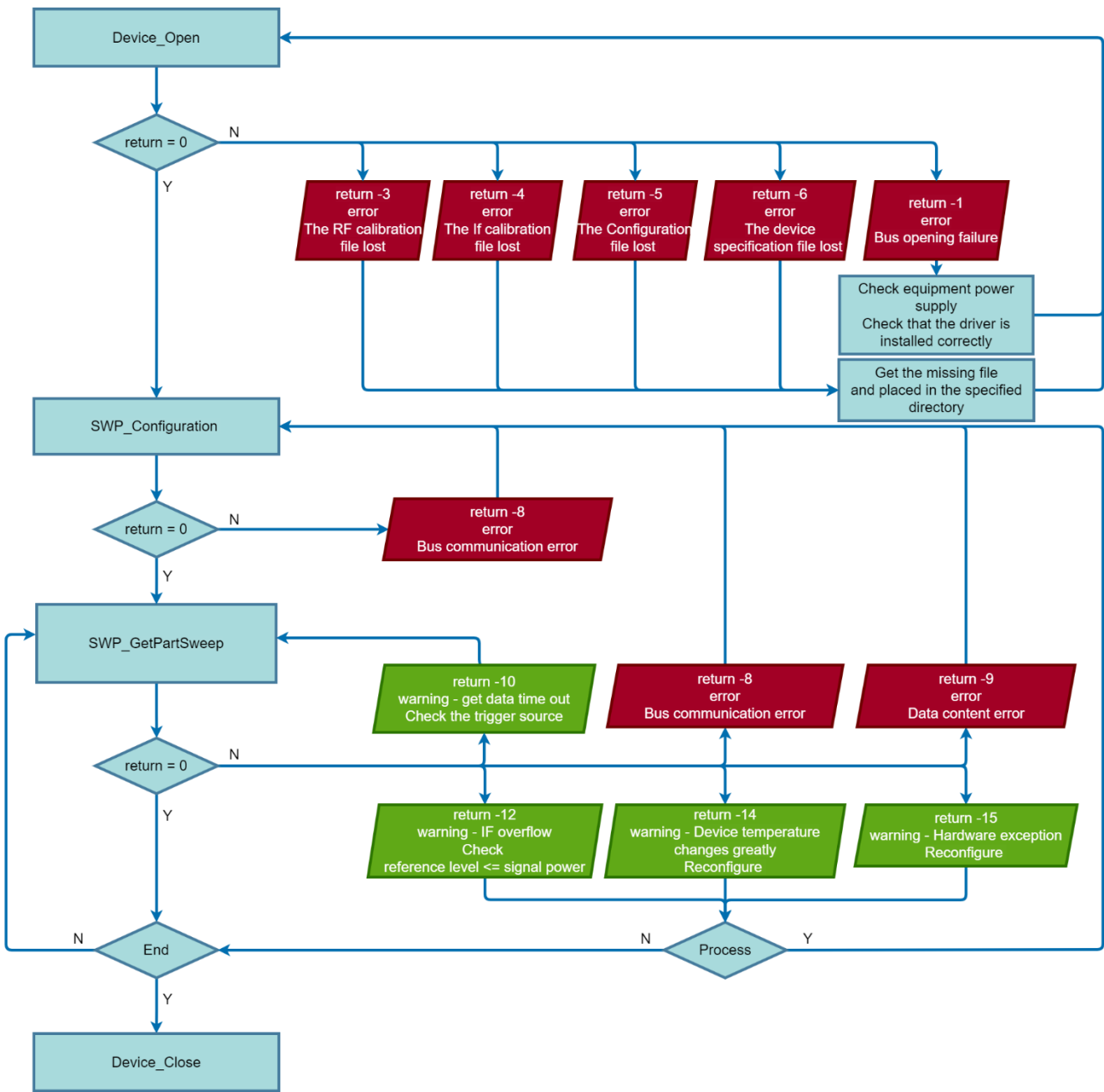
Figure 3 SWP Mode Call Flow Diagram
