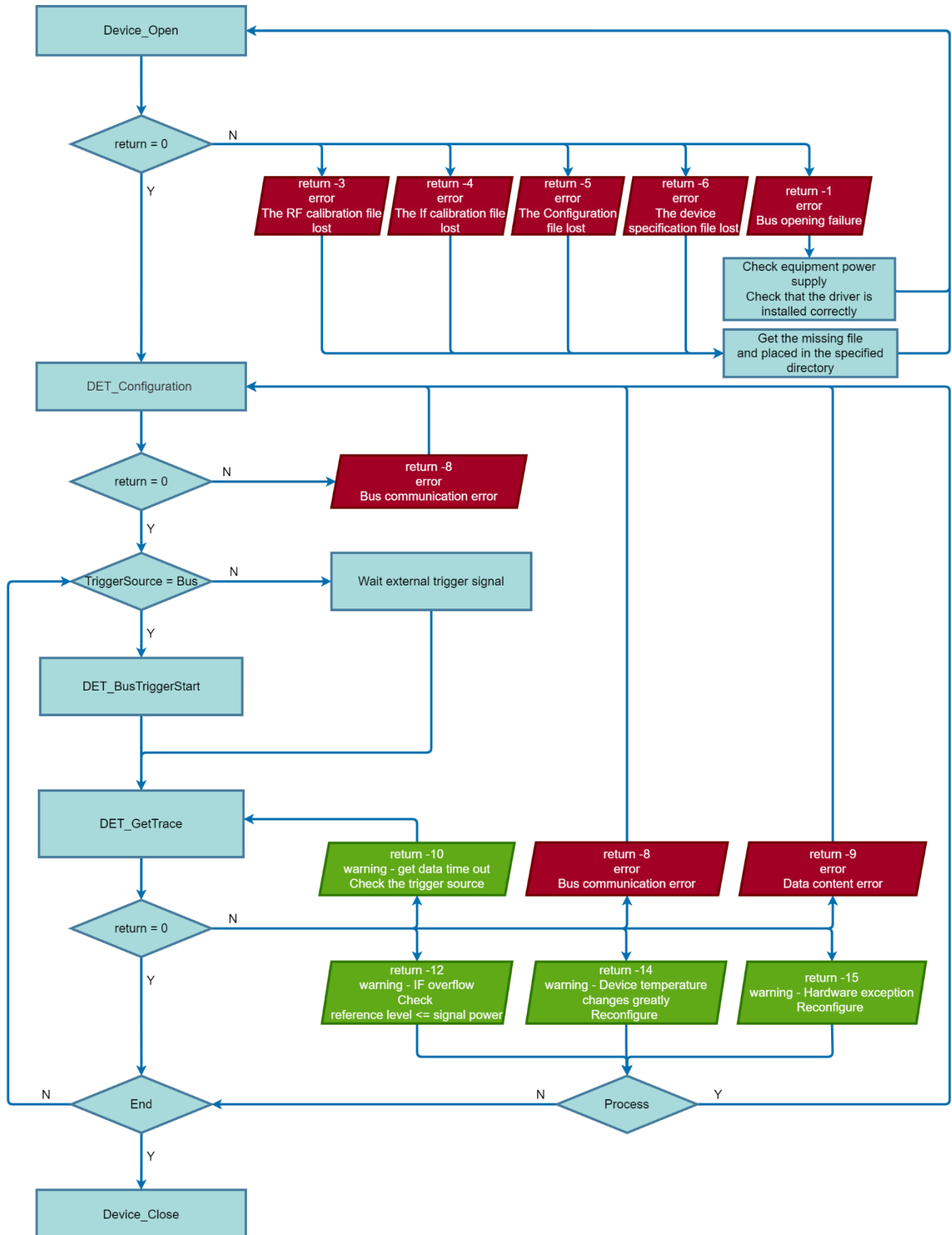
Figure 6 DET Mode Call Flow Diagram (Trigger Mode is Fixed)
