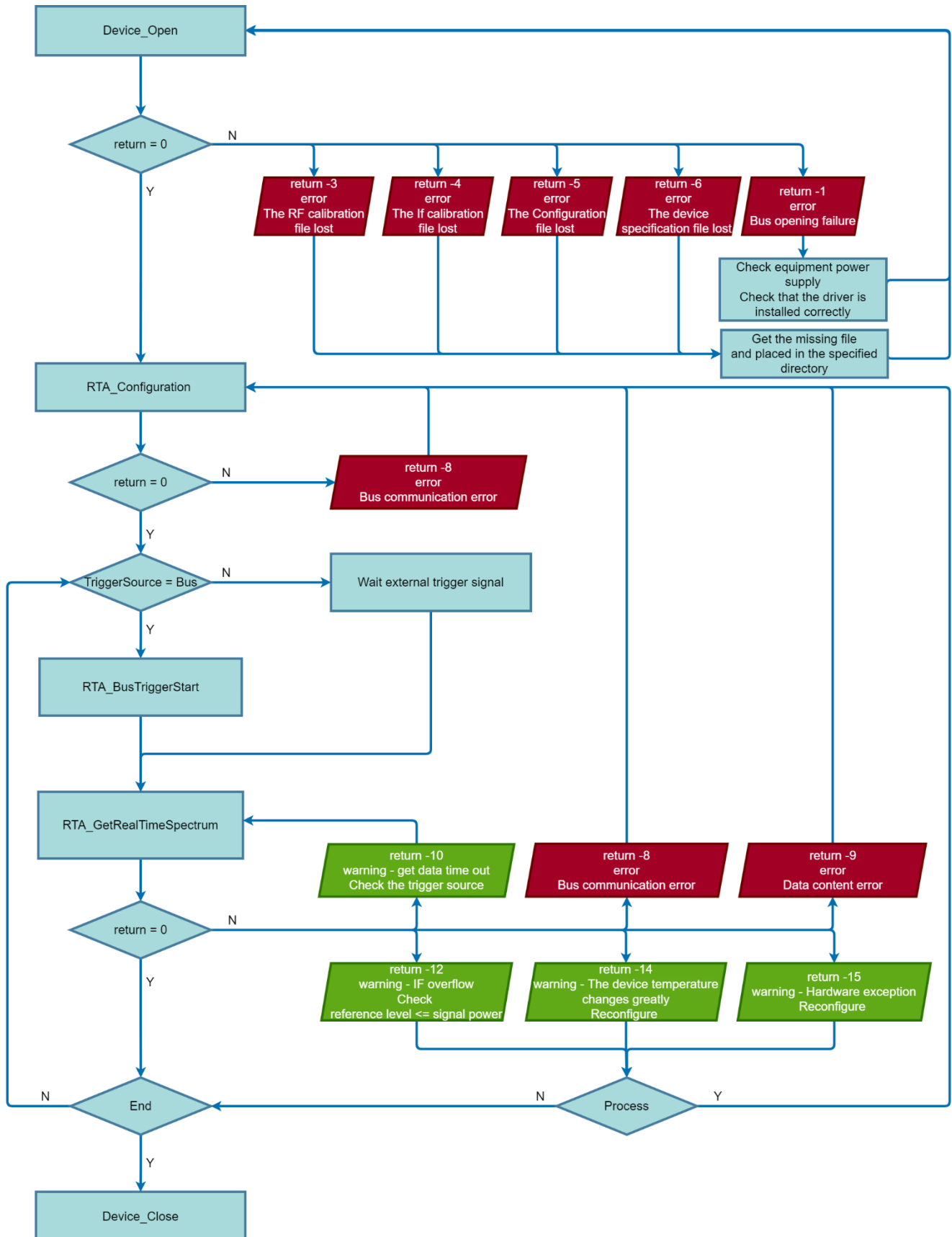
Figure 8 RTA Mode Call Flow Diagram (Trigger Mode is Fixed)
