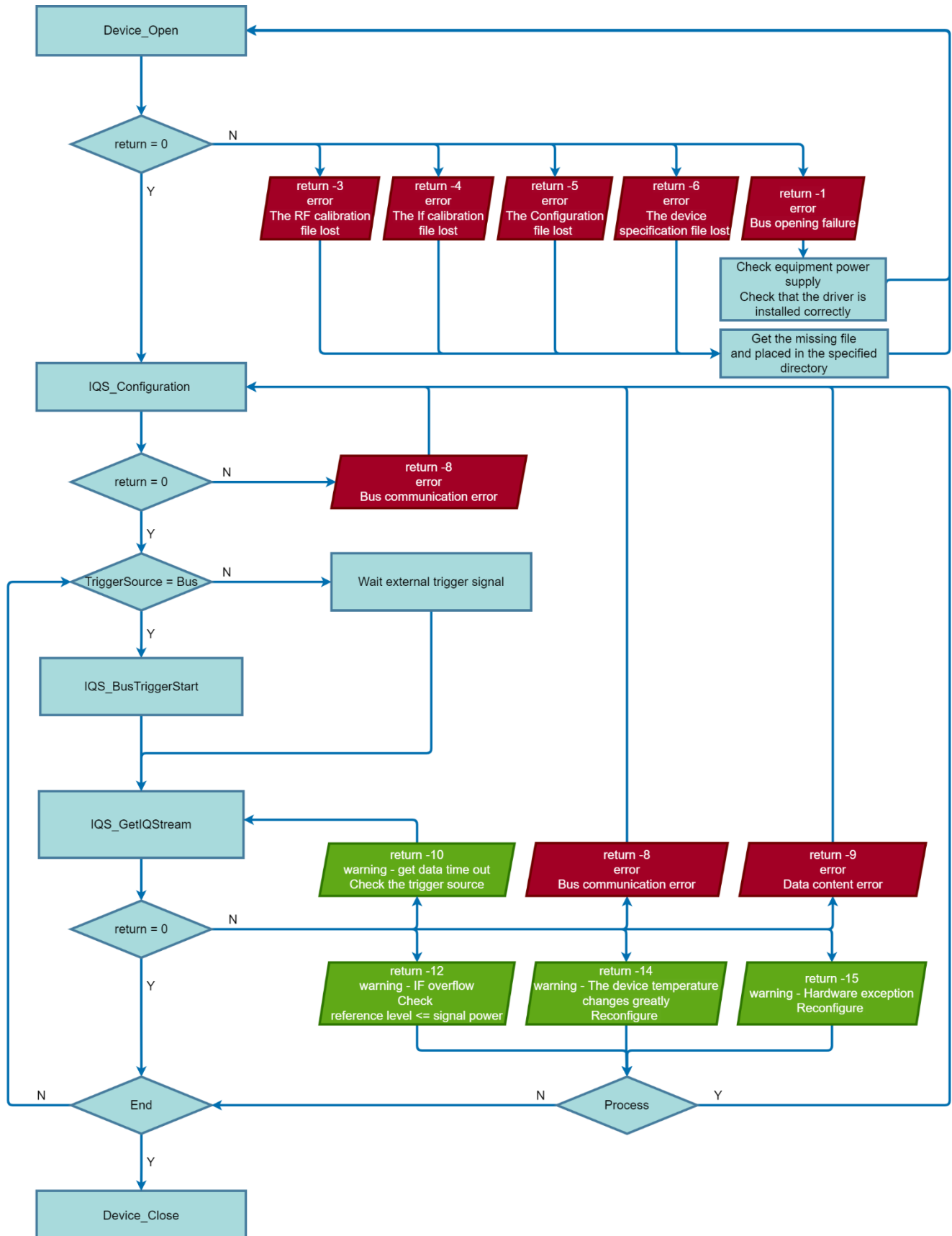
Figure 4 IQS mode Call Flow Diagram (Trigger Mode is Fixed)
