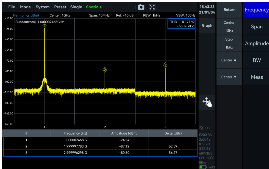
Figure 39 Measurement of Third Harmonic
