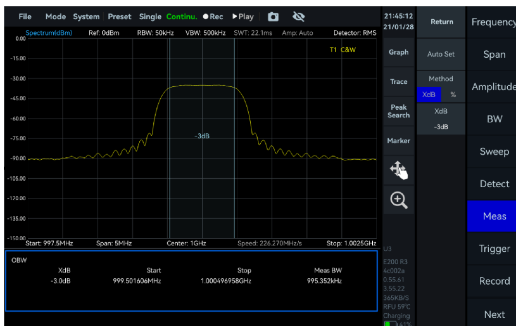
Figure 19 Measurement of OBW
